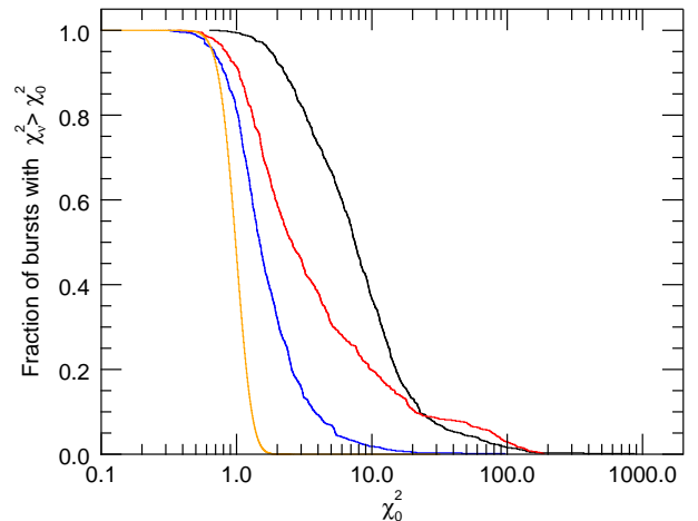
Fig. 5. Cumulative distribution for 1254 bursts of \chi_v^2 for fits with Eq. 1 (black), 2 (red), and 3 (blue). The yellow curve shows the theoretical \chi_v^2 distribution for 40 degrees of freedom (which is the average).
